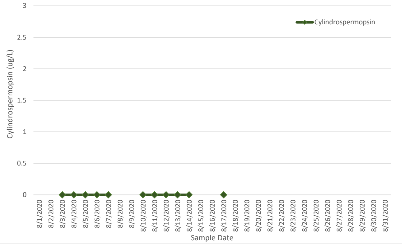
Intake - Cylindrospermopsin
