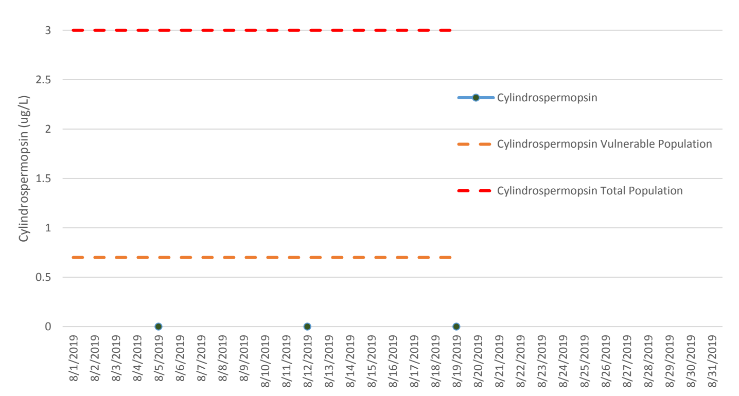
Aldersgate - Cylindrospermopsin
