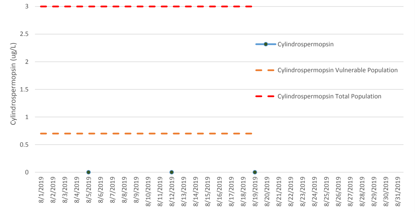
Aldersgate - Cylindrospermopsin
