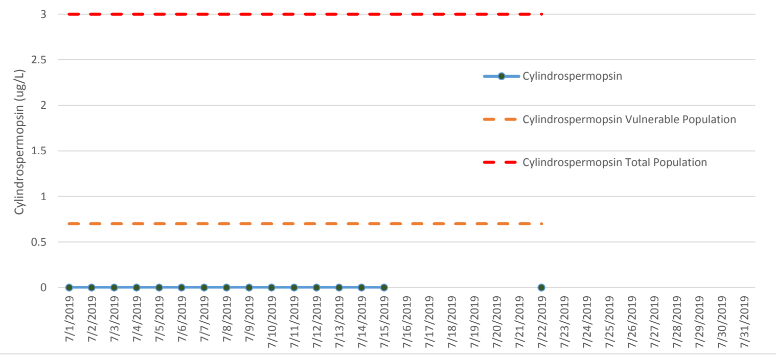
Aldersgate - Cylindrospermopsin
