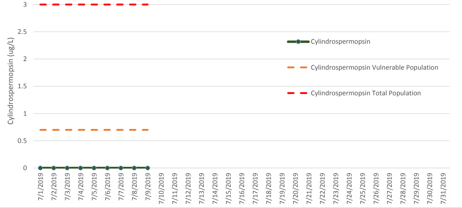
Aldersgate - Cylindrospermopsin
