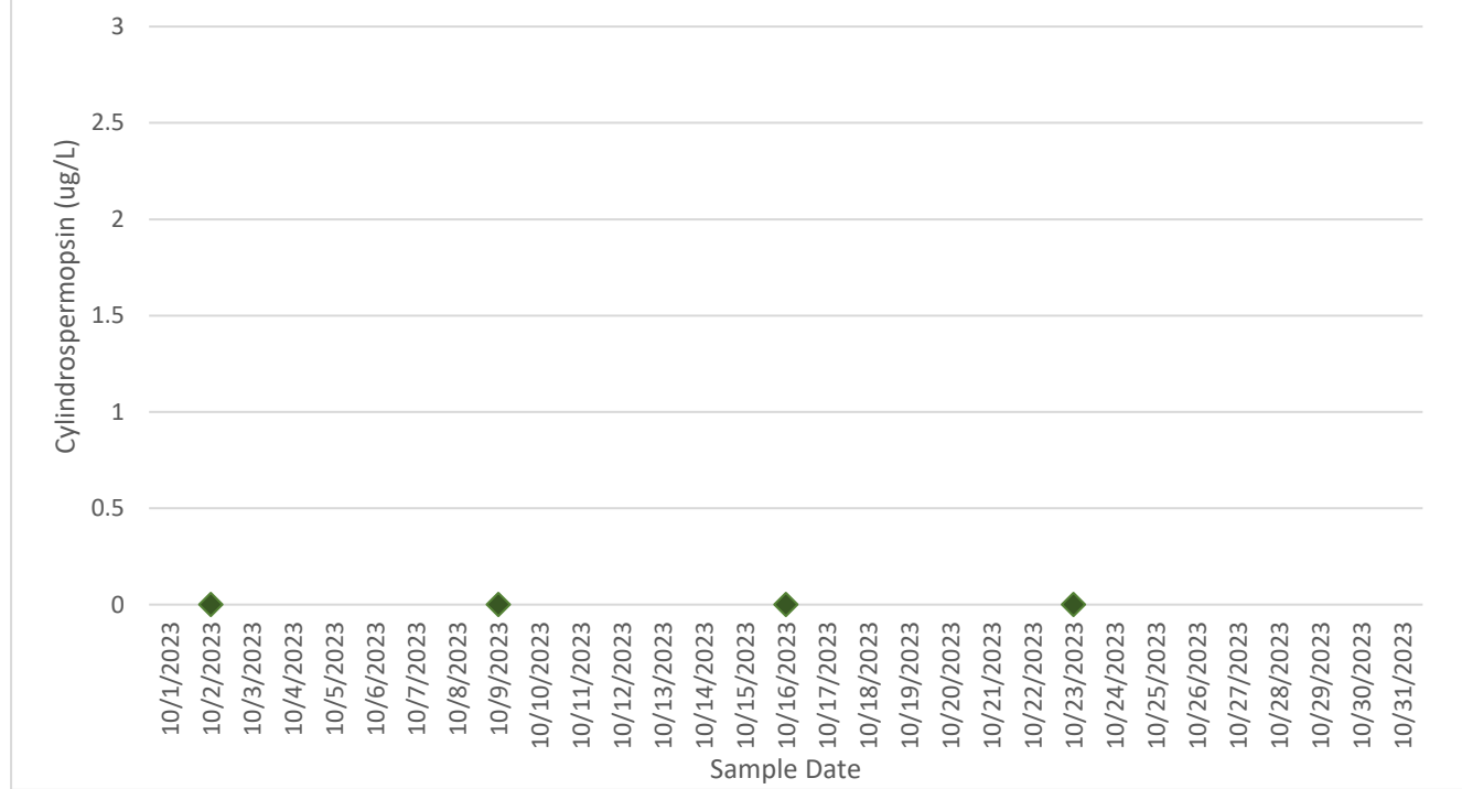
Intake - Cylindrospermopsin
