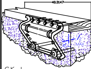
SK-1 SIMPSON STRONG-TIE UFP 10 ON A STRAIGHT FOUNDATION WITH OFFSET SILL PLATE
