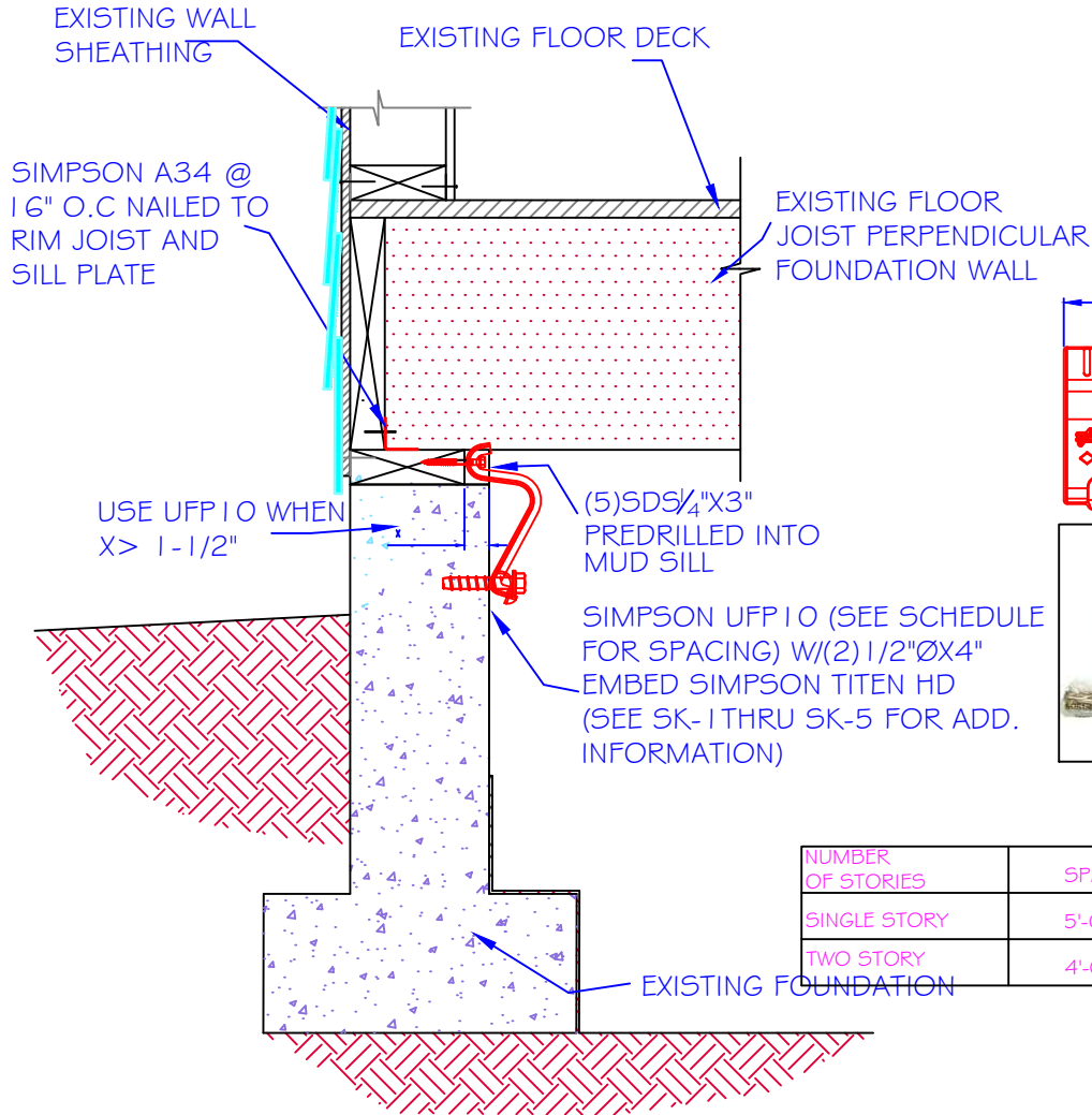
SK-5 TITEN SCREW
