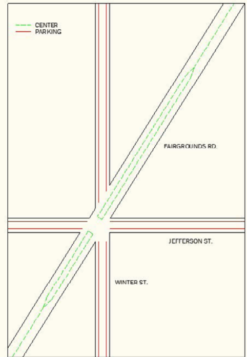
Figure 12: TWLTL design.
