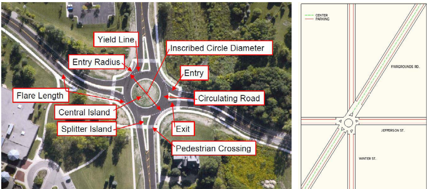
Figures 10 and 11: Example design of a roundabout; Design of roundabout option.
