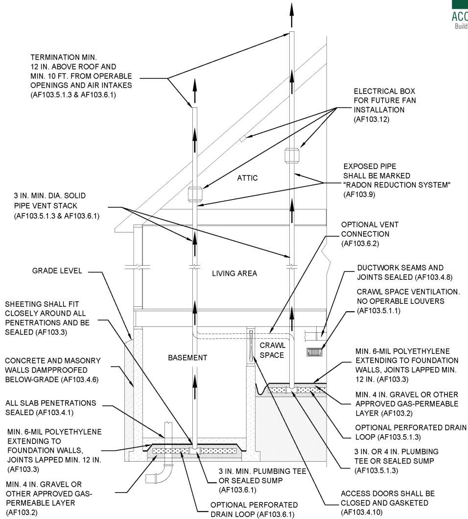
FIGURE AF103(3) RADON-RESISTANT CONSTRUCTION COMBINATION BASEMENT/CRAWL SPACE FOUNDATIONS
